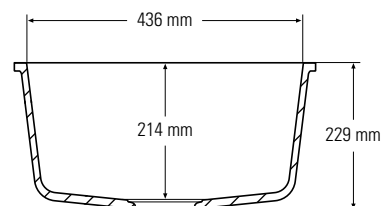
Side cross-section
