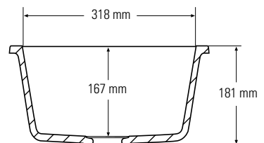
Side cross-section
