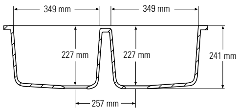
Front cross-section
