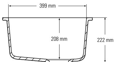
Side cross-section
