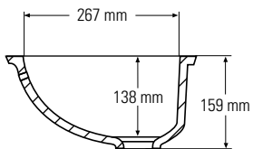
Side cross-section
