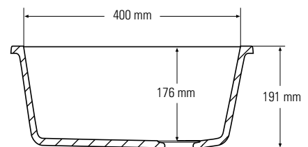
Side cross-section
