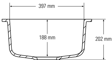
Side cross-section
