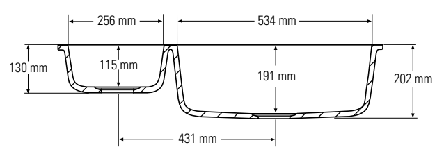
Front cross-section
