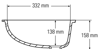
Side cross-section
