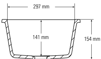
Side cross-section
