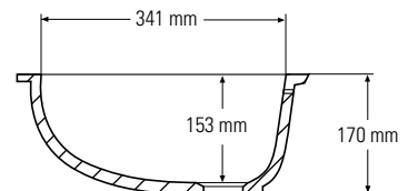
Side cross-section
