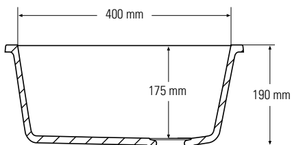
Side cross-section
