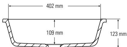
Side cross-section
